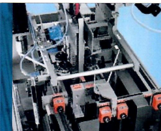
Counting stack for the infeed of blister packs
