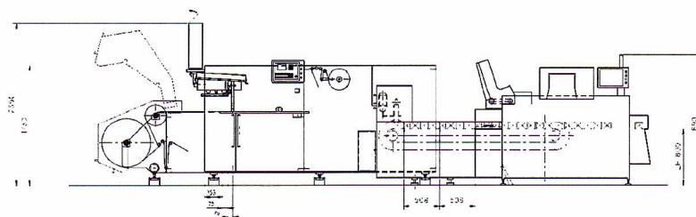
Example layout of a TLT 1400 blister machine with CUT 120 cartoning machine
