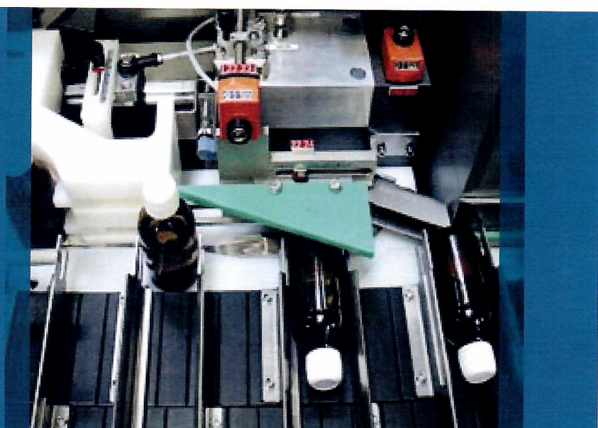
Infeed for round bottles and vials
